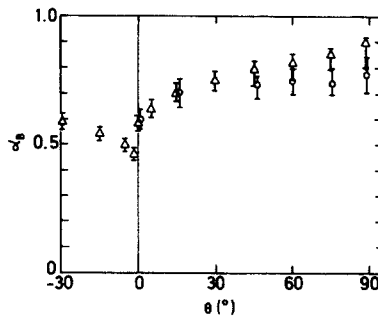
Figure 14. Measured asymptotic void fractions in the bubble for the lowest and highest liquid velocity intervals ( \Delta Fr \leq 2 , \circ Fr \geq 3.5 , D = 2.42 cm).
