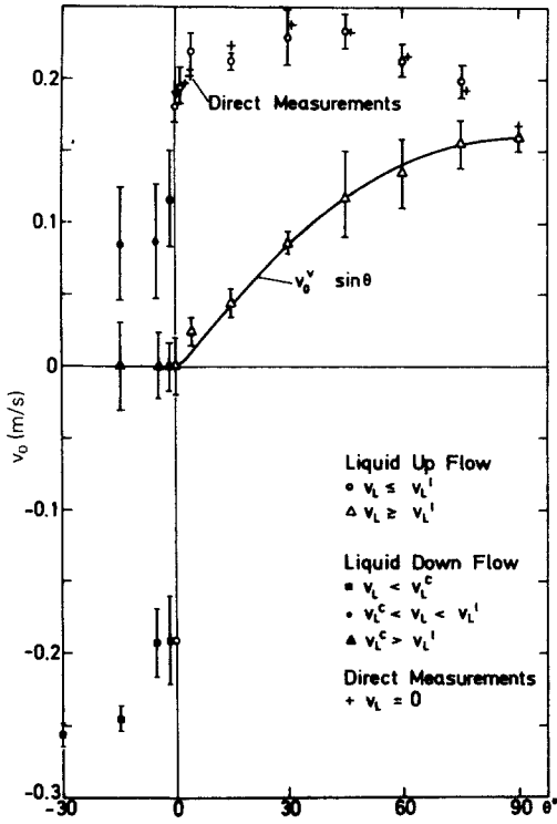
Figure 7. Bubble drift velocities in non-stationary liquid from a LSQ fit to [1] vs inclination angle with those from direct measurements in stagnant liquid (+) given as reference. ( D = 2.42 cm).
