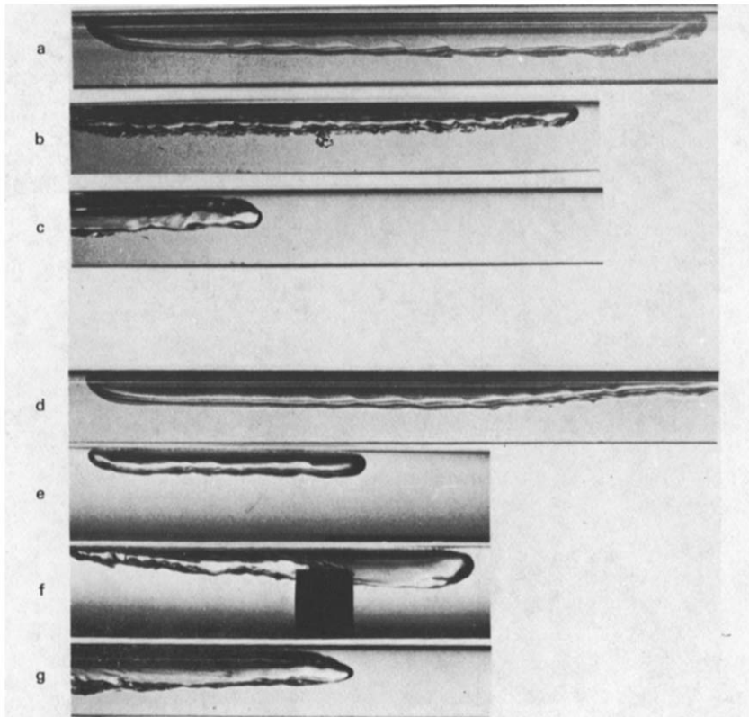
Figure 9. Illustration of the bubble turning process in liquid down flow, v_L to the right in all cases. (a-c \theta = -5^\circ , d-g \theta = -2^\circ . a, d v_L < v_L^c , b, e v_L \approx v_L^c , f v_L > v_L^c , g v_L \gg v_L^c , D = 2.42 cm).
