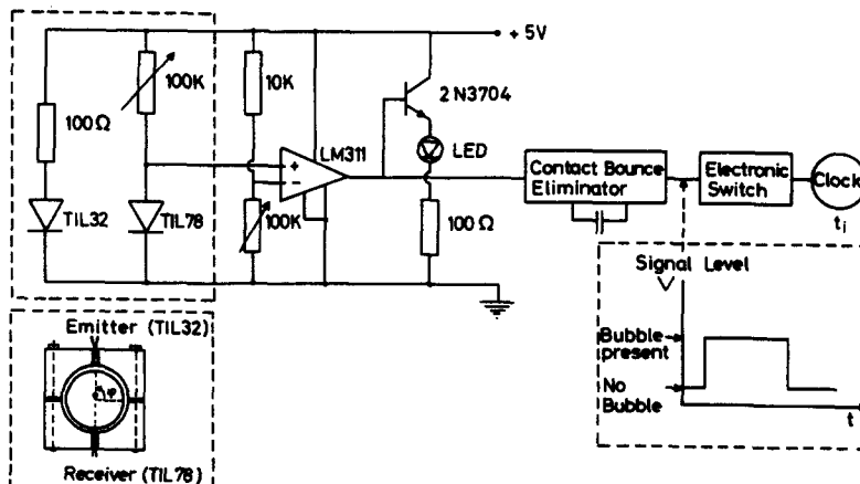
Figure 2. Schematic diagram of the bubble velocity meter.
