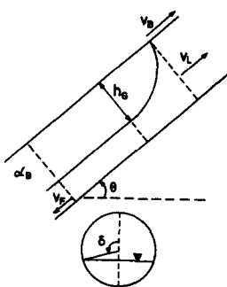
Figure 16. Schematic representation of a bubble in inclined flow ( Fr \ll 1 ).
