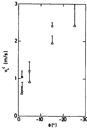
Figure 13. Critical average liquid velocities for bubble turning ( \square D = 5 cm, \circ D = 2.42 cm, \triangle D = 1.92 cm).
