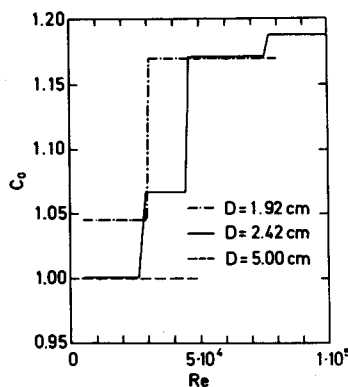
Figure 10. The coefficient C_0 vs Reynolds number for different tube diameters ( \theta = 0^\circ ).
