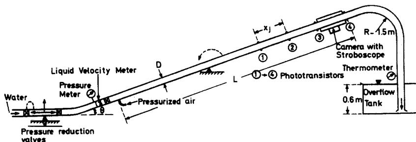
Figure 1. Schematic diagram of the test-section.
