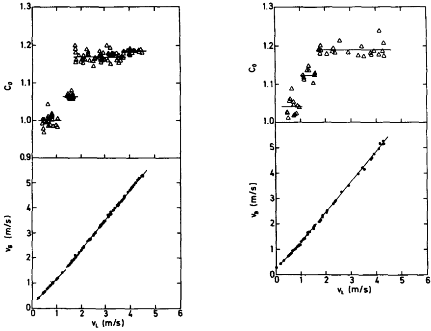
Figure 4. Measured bubble velocity and C_0 [1] vs average liquid velocity ( \theta = 0^\circ , D = 2.42 cm).
