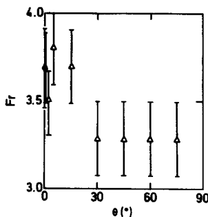
Figure 12. Froude number where transition to the highest C_0 occurs vs inclination angle ( \Delta D = 2.42 cm, \circ D = 1.92 cm).
