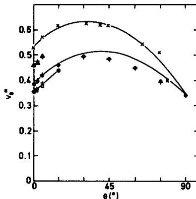
Figure 3. Dimensionless bubble propagation velocity in stagnant liquid vs inclination angle for different surface tension parameters (—[10], Our data: \square , \circ , \triangle , \Sigma = 0.064, 0.042, 10^{-2} . Data of Zukoski (1965): \times \Sigma = 10^{-3} , + \Sigma = 10^{-2}, 0.042, 0.064 ).
