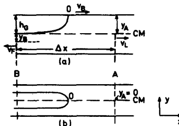
Figure 15. Schematic representation of a bubble in horizontal flow ((a) Fr \leq 1 , (b) Fr \geq 1 ).
