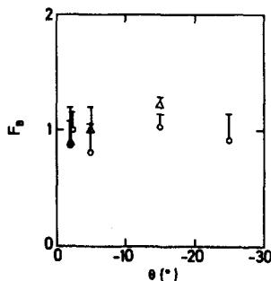
Figure 17. Measured bubble turning velocities represented by the F_B -number [17] ( \circ D = 1.92 cm, \triangle D = 2.42 cm, \square D = 5.00 cm).
