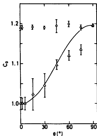
Figure 11. The coefficient C_0 vs inclination angle for the lowest ( \Delta ) and highest ( \circ ) velocity intervals ( D = 2.42 cm, — C_0(\theta) = (C_0(0^\circ) + [C_0(90^\circ) - C_0(0^\circ)] \cdot \sin^2 \theta) ).
